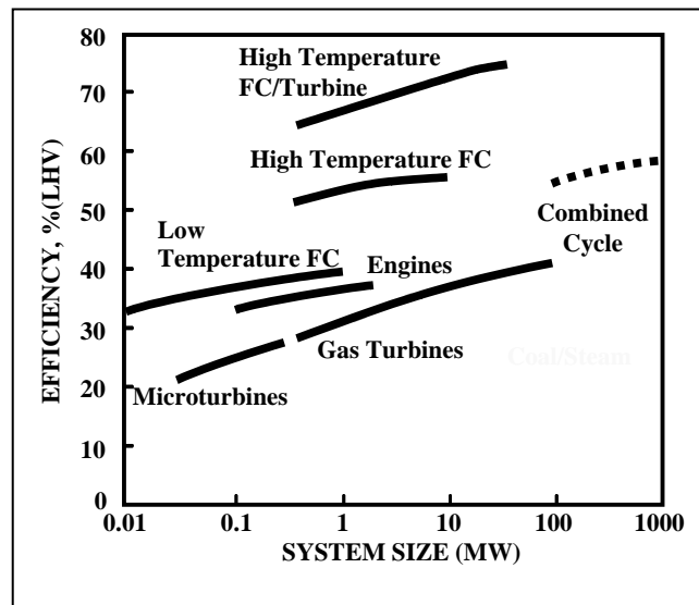
Figure 5. Electrical System Efficiencies of Fuel Cells Compared with Other Electric Power Plants
