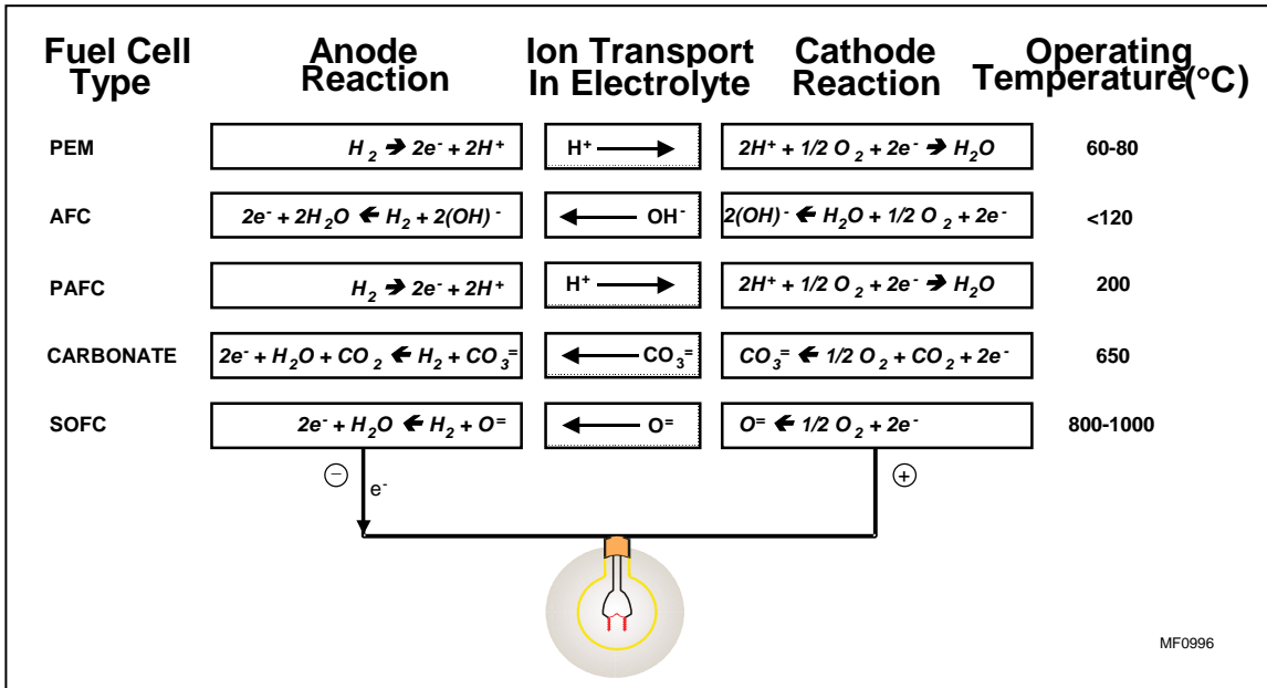
Figure 1. Schematic of Different Fuel Cell Types
