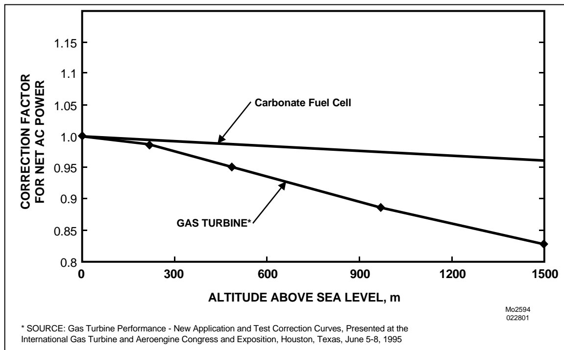
Figure 6. Comparative Example of Relatively Negligible Effects of Ambient Temperature and Altitude on Fuel Cell Performance
