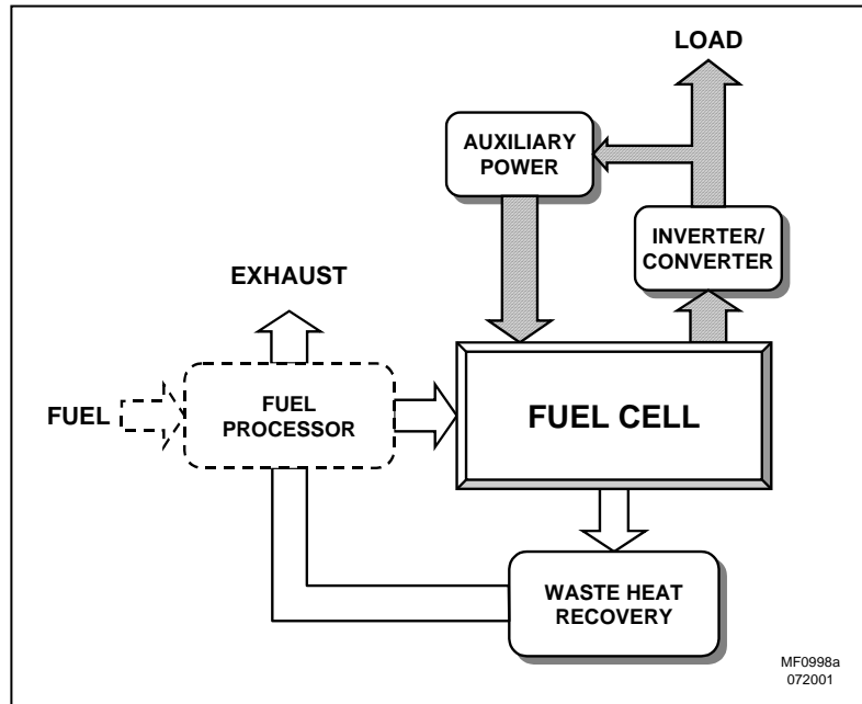
Figure 2. Basic Fuel Cell System
