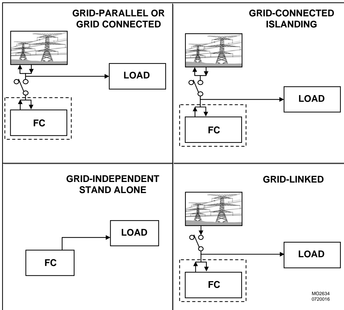
Figure 7. Schematic Illustrating Various Fuel Cell System Power Electronic Configurations
