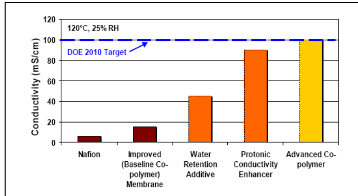
Figure 1. DEVELOPMENTS STEPS TO THE CONDUCTIVITY GOAL: Each Individual Component Contributes to Conductivity Improvements.
